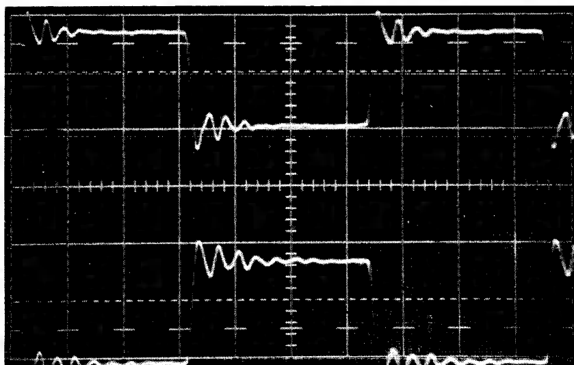
FIGURE 3.6a – Improper Clocks (Note undershoot and overlap)
